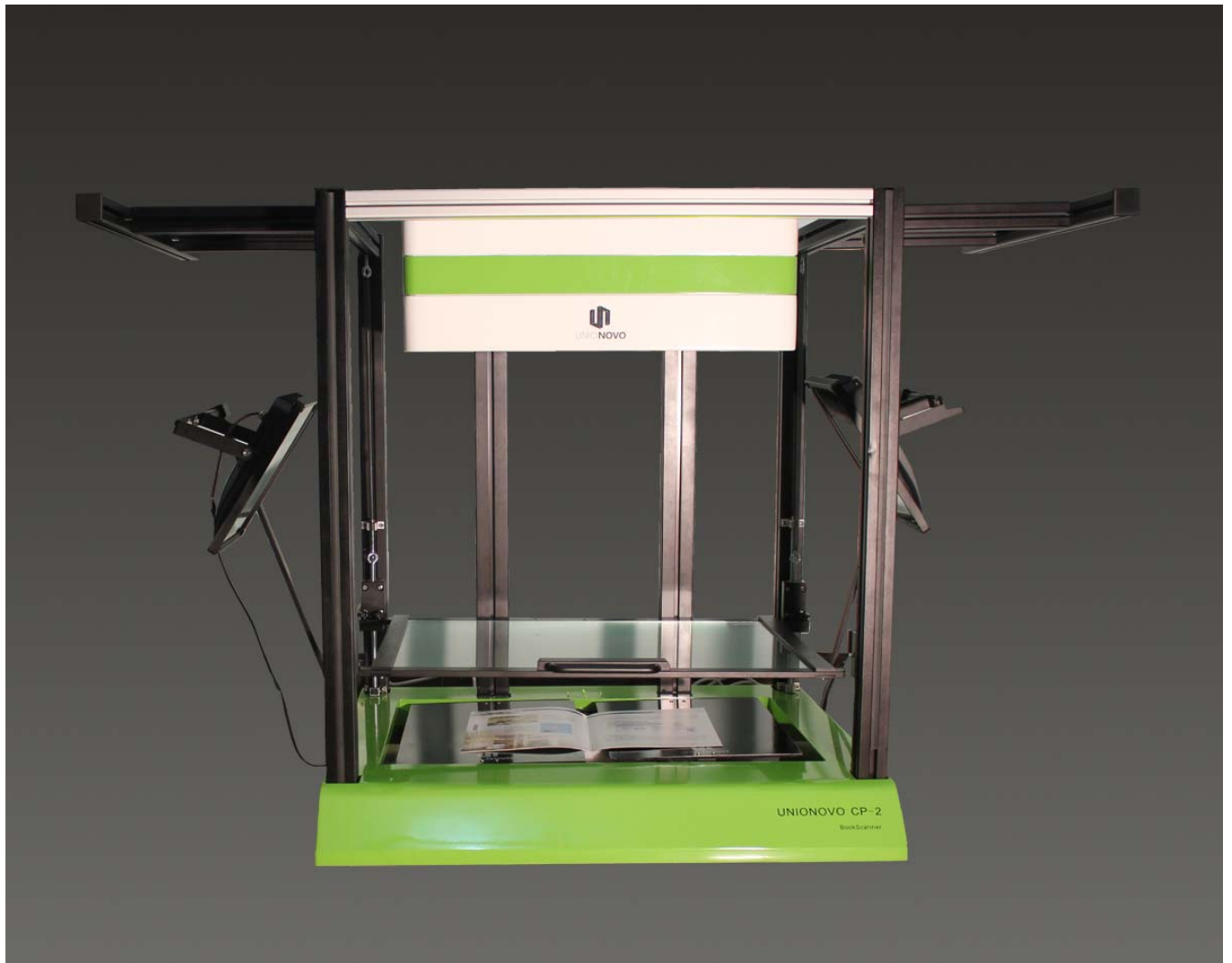
A2+ TOP professional high-speed book scanner
